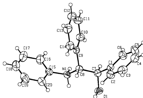
Figure 2. ORTEP diagram (40% probability factor for the thermal ellipsoid) of the cationic part of compound (1 R ,2 R )-diphenyl-2-(phenylamino)ethanol hydrochloride with atom-numbering scheme.
