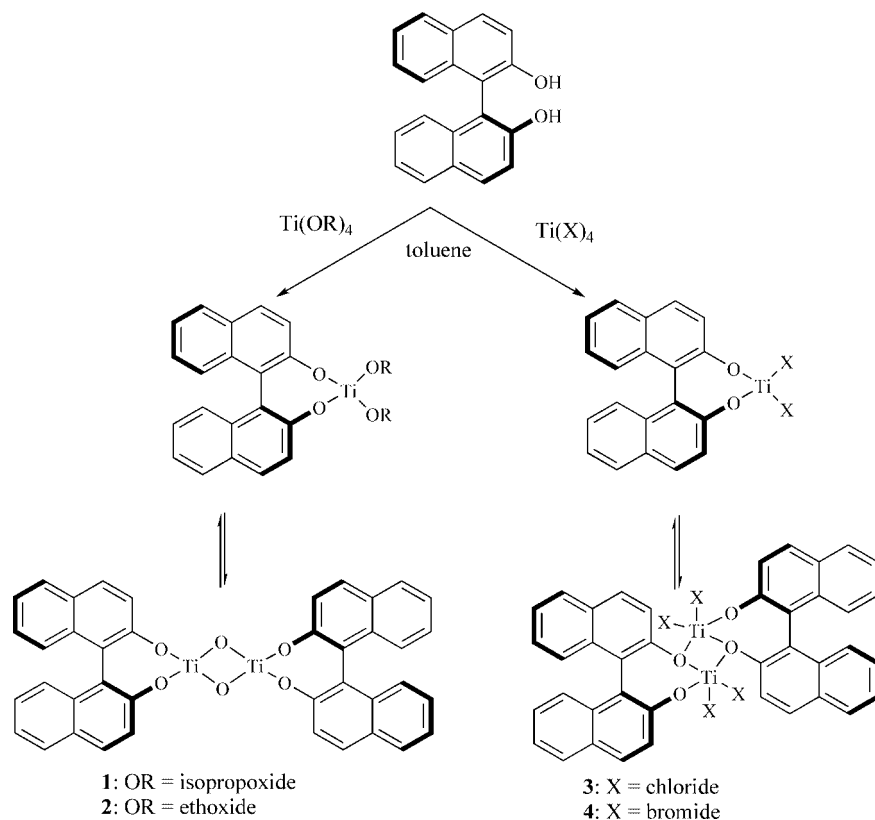
Scheme 1. Synthesis of catalyst 1–4.
