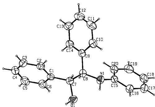
Figure 1. ORTEP diagram (40% probability factor for the thermal ellipsoid) with atom-numbering scheme for racemic 1,2-diphenyl-2-(phenylamino)ethanol.
